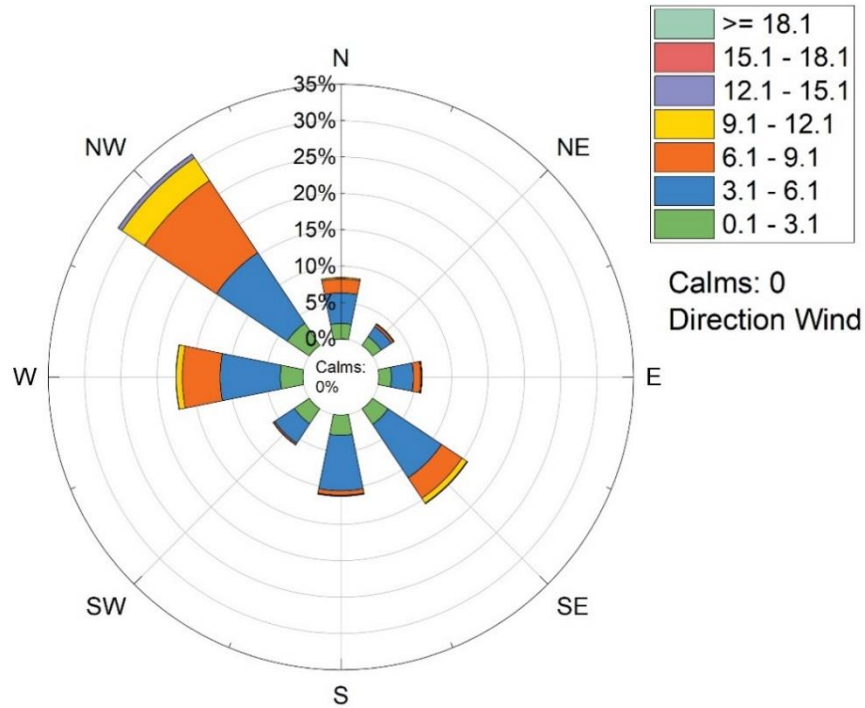
Figure (2) Wind Rose for Year 2022
