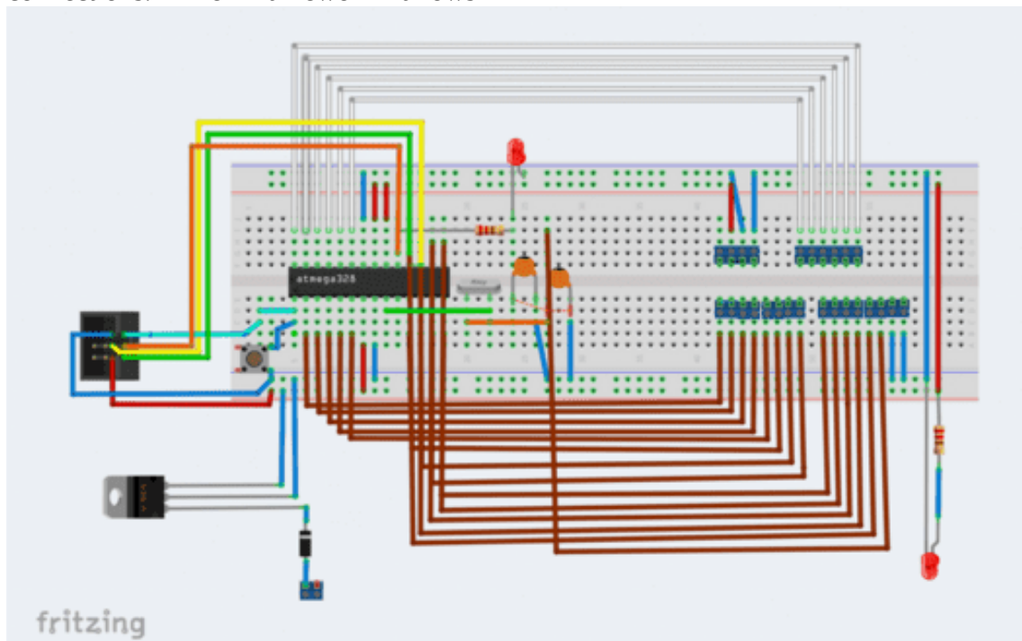
Figure (2) Breadboard Connection.
